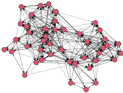
Fig. 1. Friendship network
