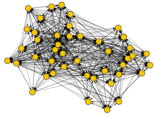
Fig. 2. Advice network
