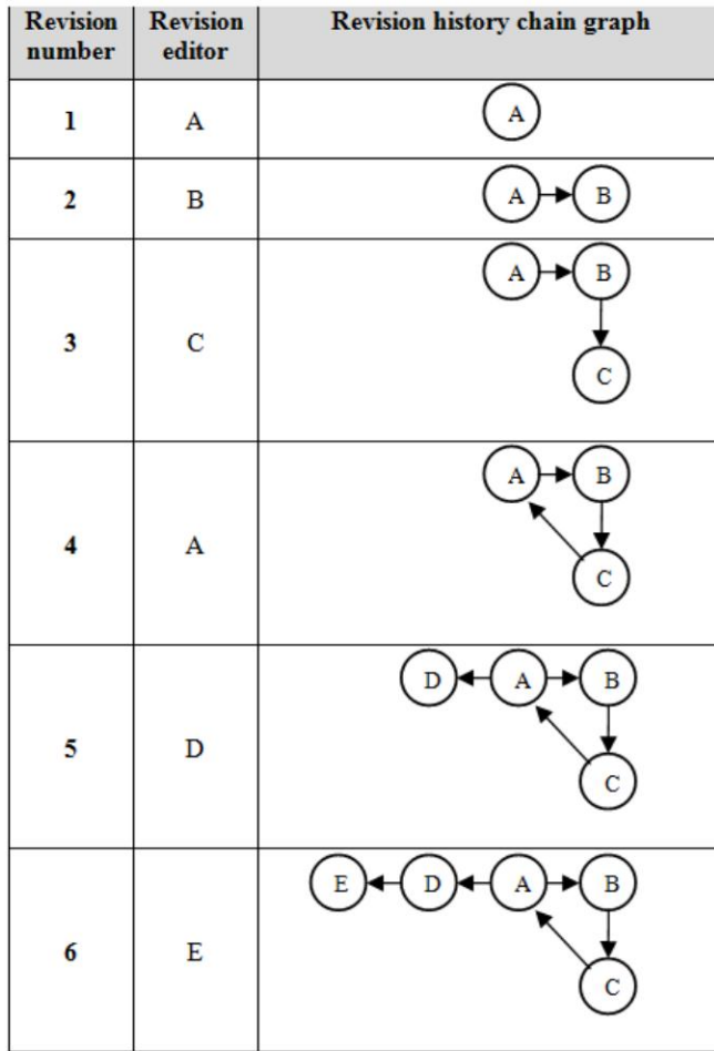
Figure 1: Article trajectory construction example
