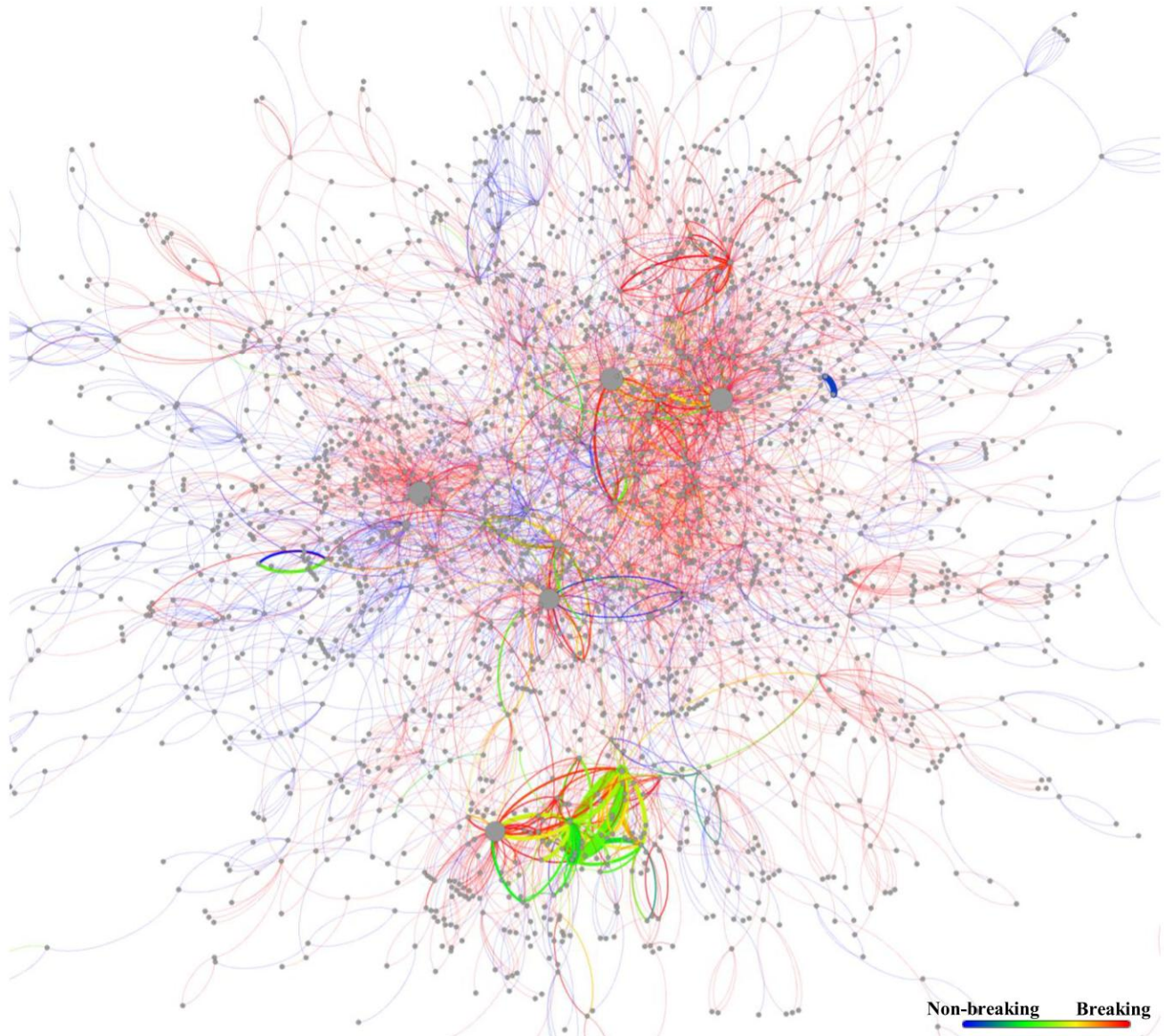
Figure 3: Largest component in repeat interaction multigraph. Editors (in grey, sized by degree) are linked with weighted edges if their interactions with another editor appear on two or more distinct articles. Bluer edges have greater fractions of non-breaking article interactions, redder edges have greater fractions of breaking article interactions.
